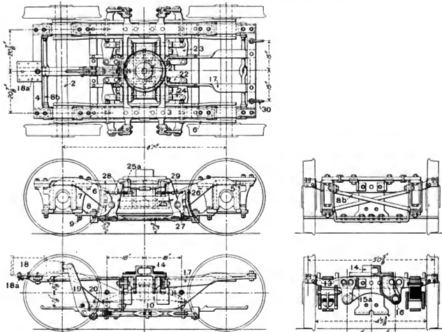
Figs. 3376-3380. Swing Motion Four-Wheel Front Engine Truck with T Hangers. Atlantic (4-4-2) Locomotive. Pennsylvania Railroad.
